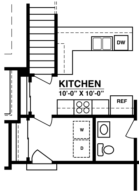
OPTIONAL KITCHEN #2
